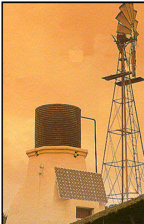
PV - Wind Hybrid Water Pumping
